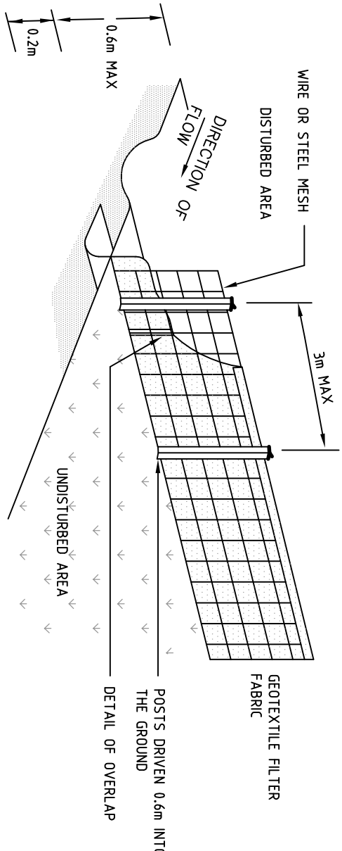
DETAIL A SEDIMENT CONTROL FENCE SCALE: NTS
